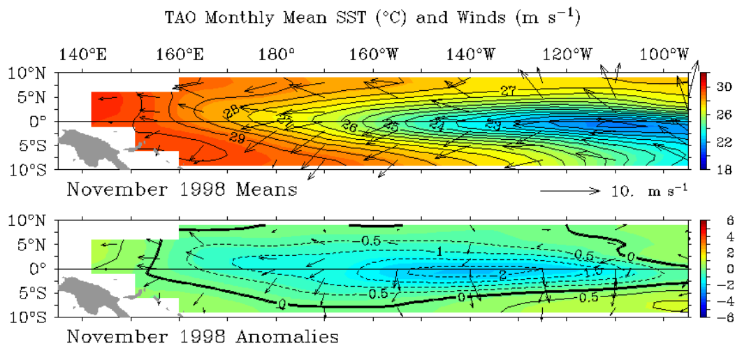
Figure 8. TAO data averaged for the month of November 1998 . The upper panel shows observed mean sea surface temperature and wind flow. The color scale on the right indicates temperature in ^{\circ}\text{C} . The direction of the wind arrow indicates wind flow direction and the length of the arrow indicates wind strength (in meters per second). The lower panel shows sea surface temperature anomalies and wind anomalies for November 1998. Image courtesy NOAA / PMEL / TAO Project Office.
