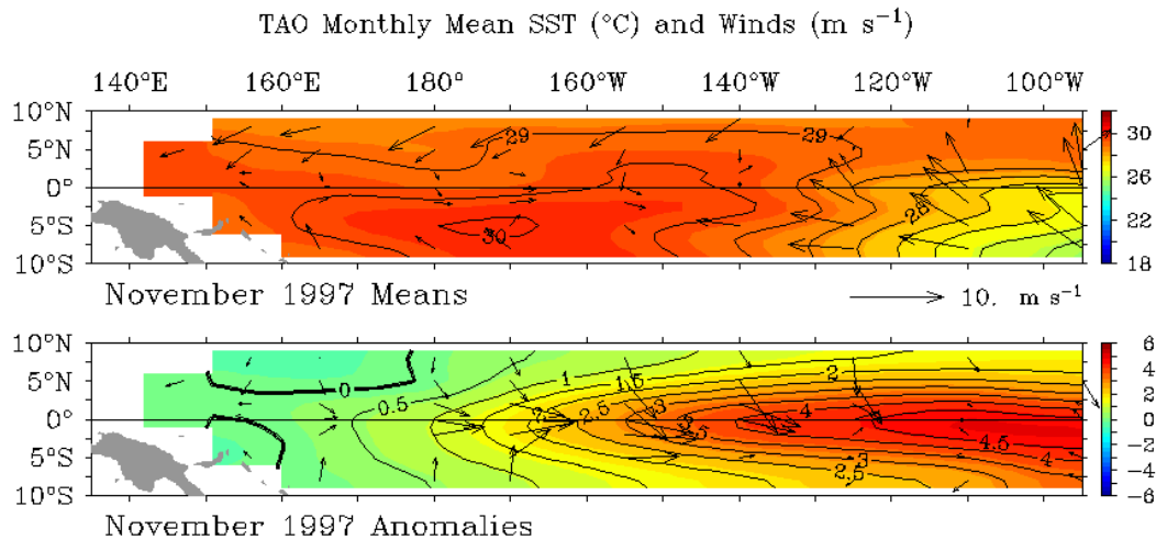
Figure 7. TAO data averaged for the month of November 1997 . The upper panel shows observed mean sea surface temperature and wind flow. The color scale on the right indicates temperature in ^{\circ}\text{C} . The direction of the wind arrow indicates wind flow direction and the length of the arrow indicates wind strength (in meters per second). The lower panel shows sea surface temperature anomalies and wind anomalies for November 1997. Image courtesy NOAA / PMEL / TAO Project Office.
