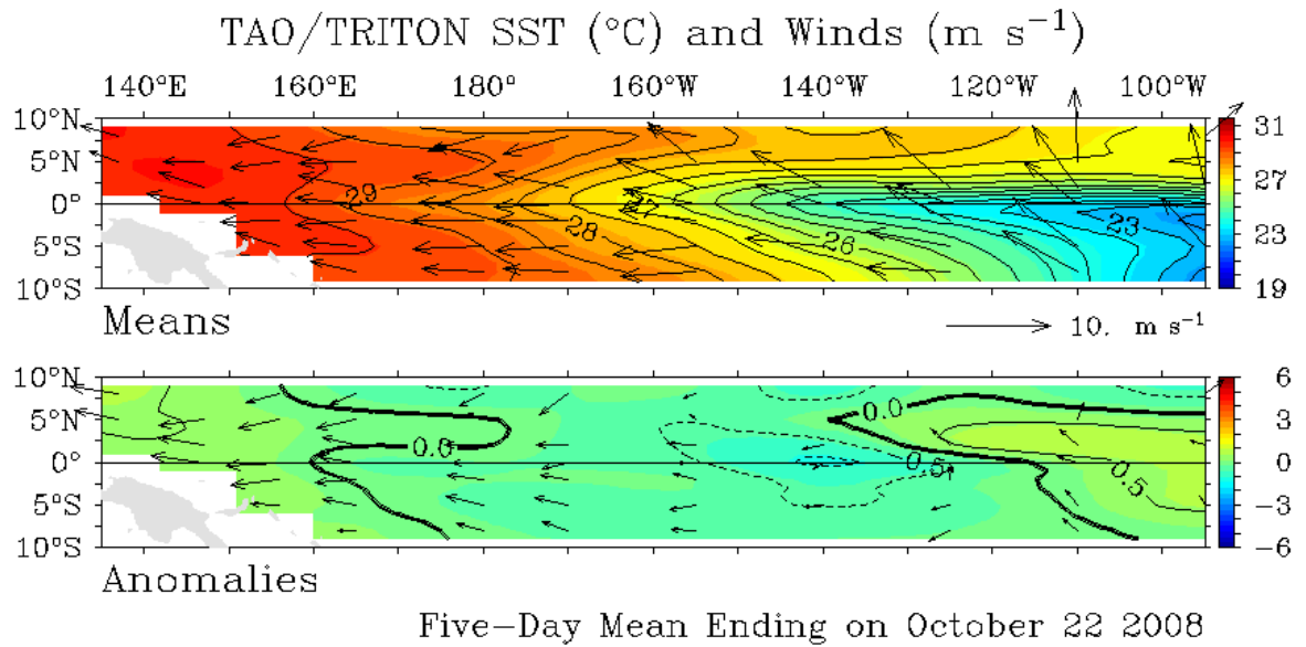
Figure 6. TAO/TRITON data for a period of five days ending October 22, 2008. Data is shown as a five-day mean (average). The upper panel shows observed sea surface temperature and wind flow. The color scale on the right indicates temperature in ^{\circ}\text{C} . The direction of the wind arrow indicates wind flow direction and the length of the arrow indicates wind strength (in meters per second). The lower panel shows sea surface temperature anomalies and wind anomalies. Image courtesy NOAA / PMEL / TAO Project Office.
