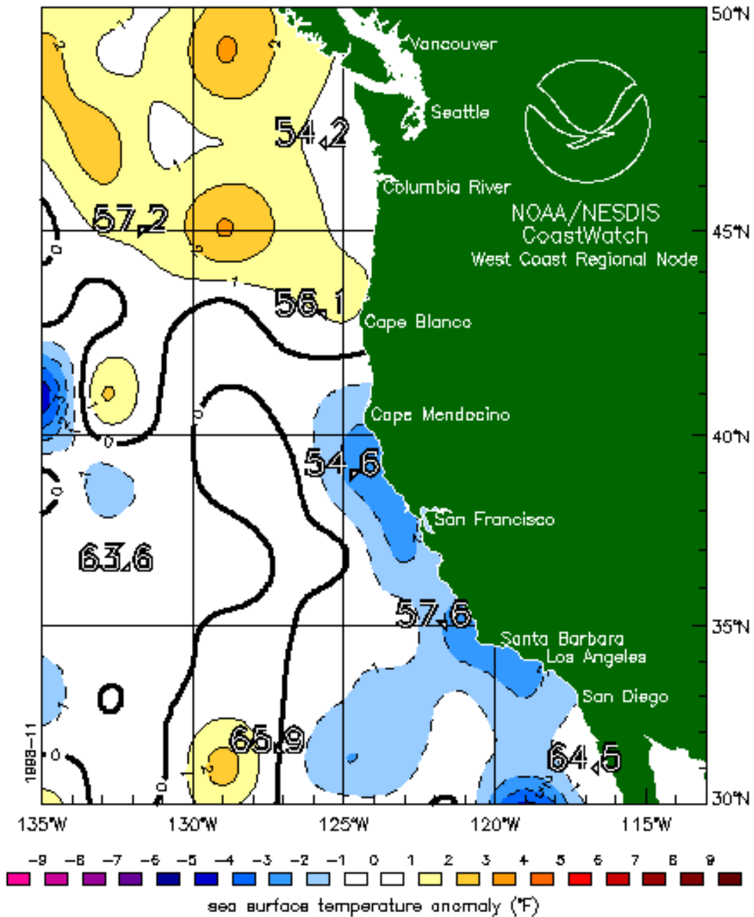
Figure 12. CoastWatch Advisory for November, 1998. In this image, coastal ocean mean sea surface temperatures (°F) are shown as the large numbers. Sea surface temperature anomalies are shown as contoured and color-coded values. Upwelling along the central and Southern California coast was observed to be slightly above normal at this time.
